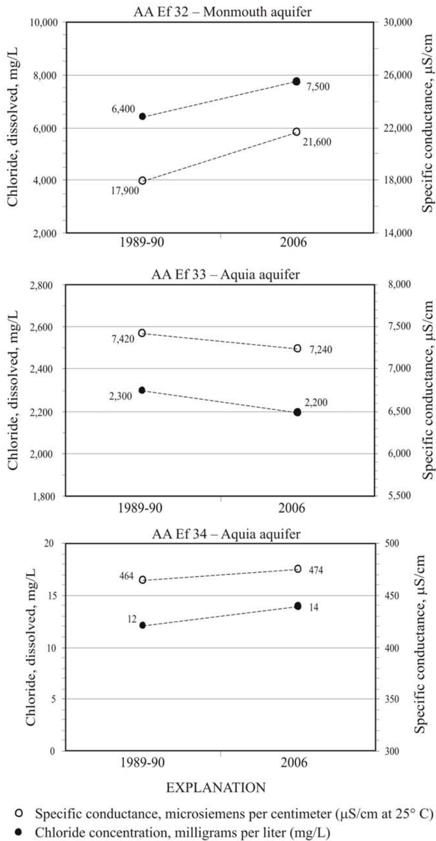
Figure 9. Change in dissolved chloride and specific conductance between 1989-90 and 2006 at Mayo Beach Park test site.
