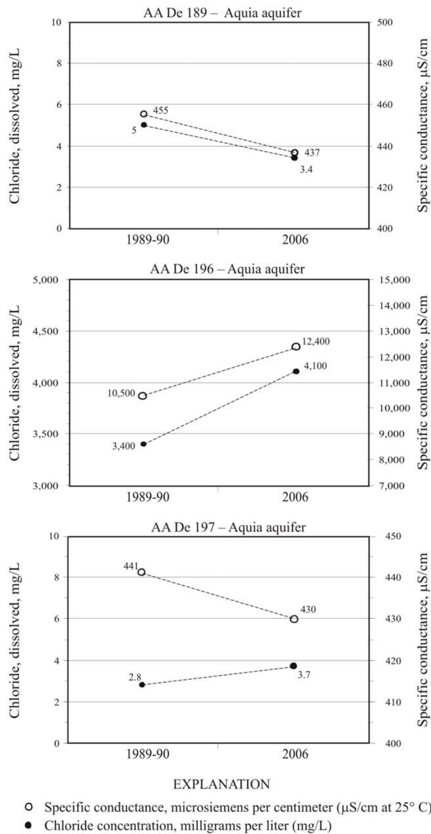
Figure 4. Change in dissolved chloride and specific conductance between 1989-90 and 2006 at Quiet Waters Park test site.
