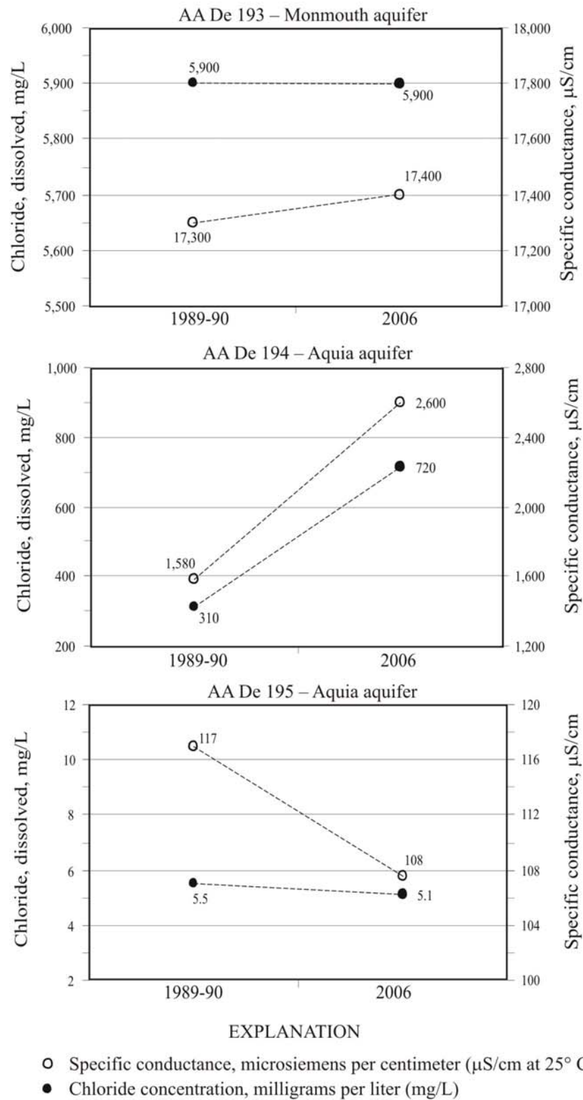
Figure 5. Change in dissolved chloride and specific conductance between 1989-90 and 2006 at Londontown Park test site.
