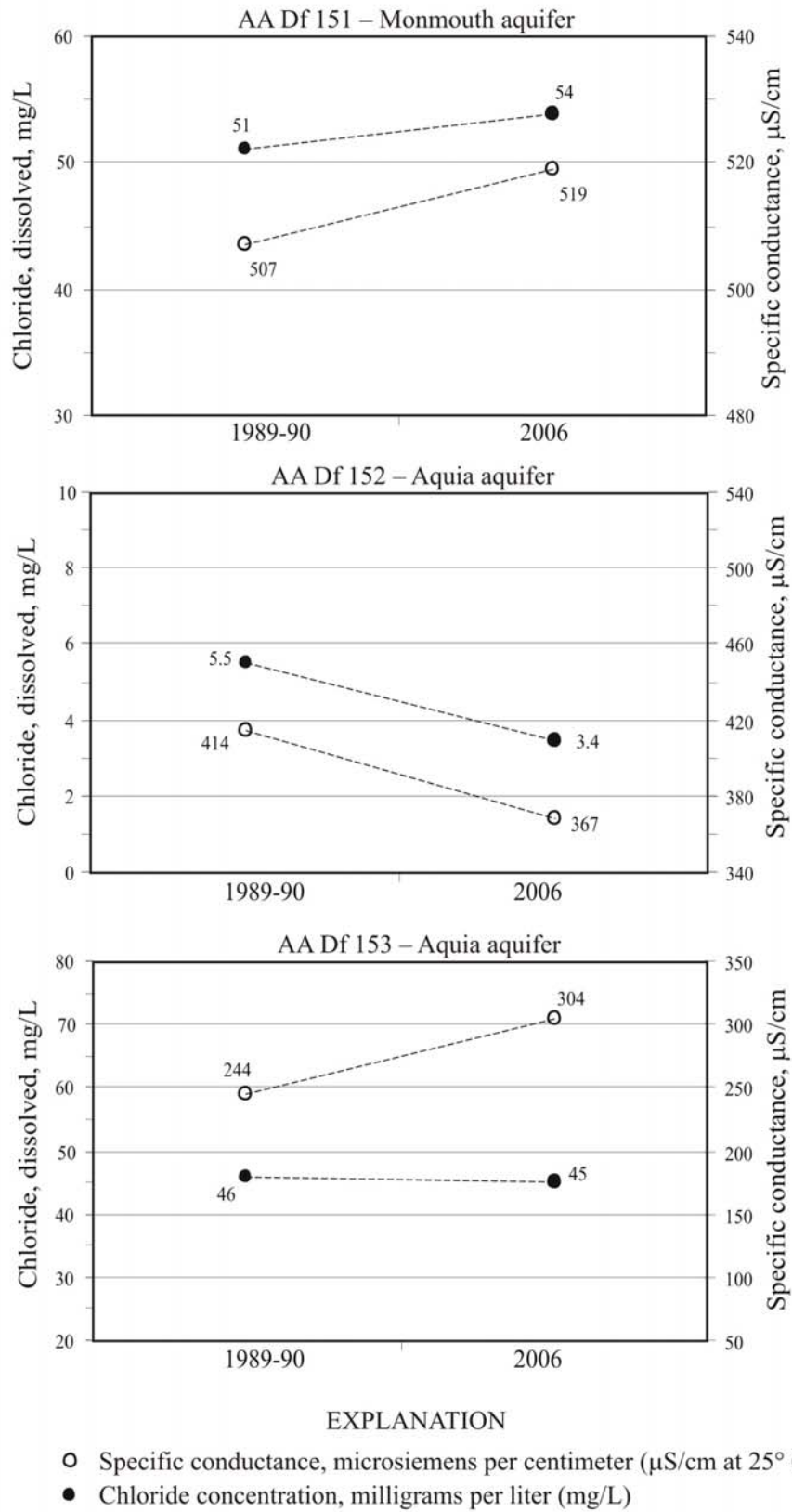
Figure 6. Change in dissolved chloride and specific conductance between 1989-90 and 2006 at Annapolis Roads test site.
